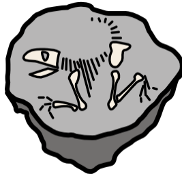
fossil
