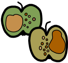
decomposition
