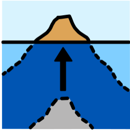
emerge
