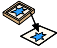
rock imprinting
