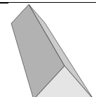
triangular prism
