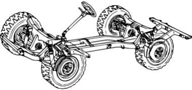
chassis
