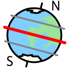
equator
