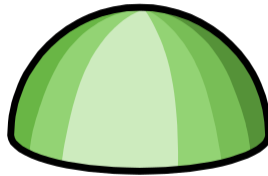
hemisphere
